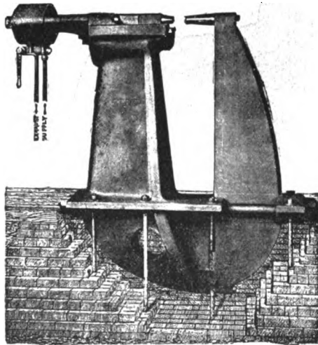
FIG. 98.—HYDRAULIC RIVETER.
